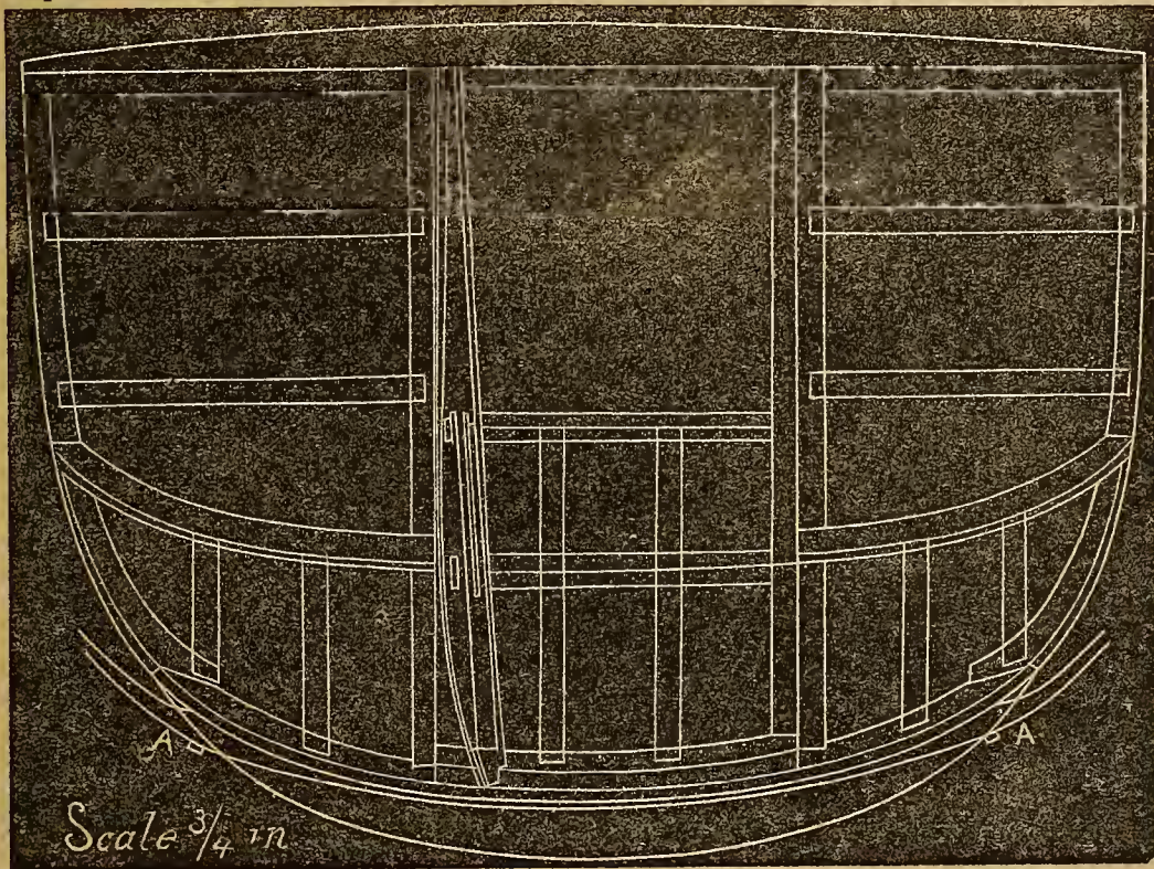
FRAME-WORK OF THE ROUND-BODIED COACH ON PLATE VIII.
